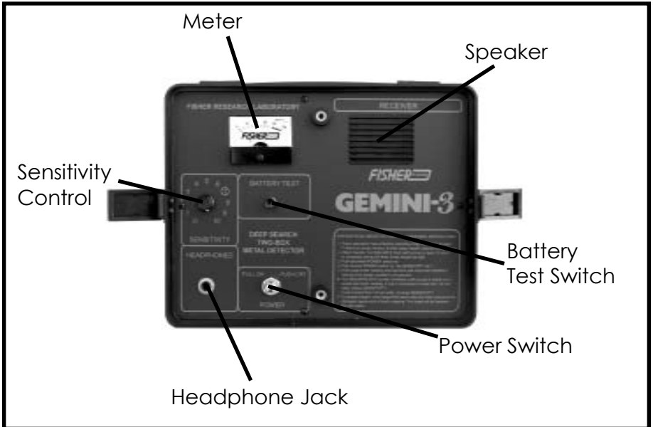
Figure 3. Receiver
